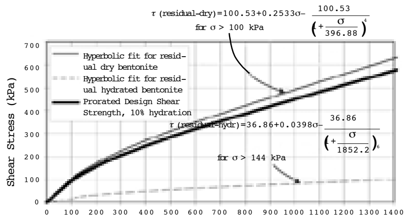
Figure 5: Prorated shear-strength curve for encapsulated, partially hydrated bentonite.
