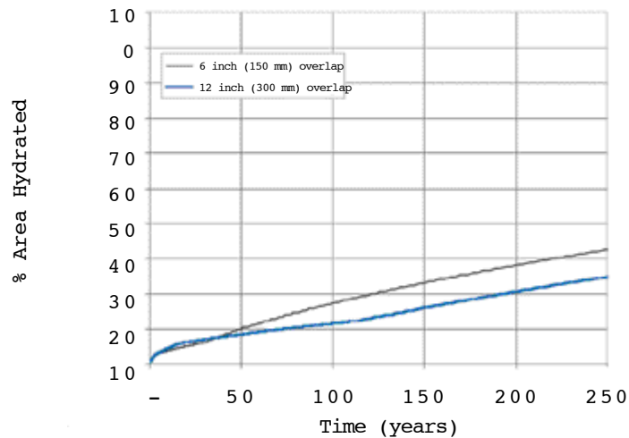
Figure 4: Predicted percent area hydrated of the encapsulated bentonite coating of the GM-GCL through overlaps deployed on a wet subgrade.
