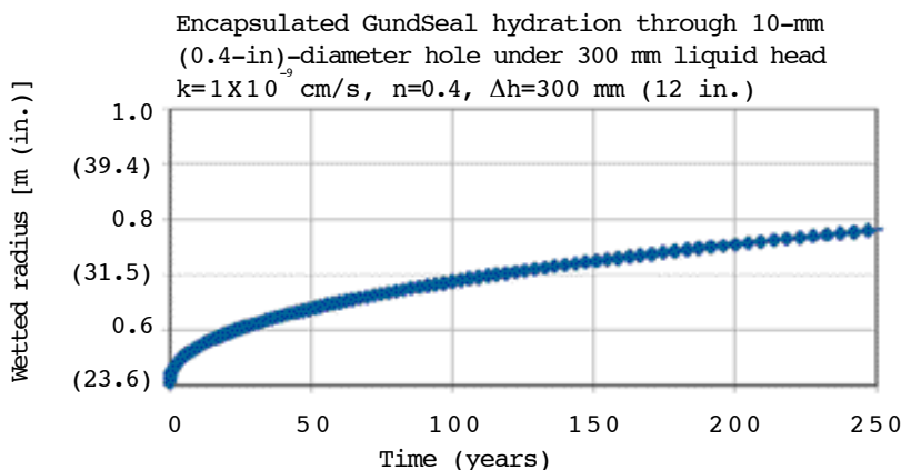
Figure 3: Predicted wetting of the encapsulated bentonite through a single 10-mm-diameter defect in a geomembrane.
